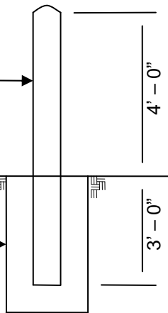
SECTION VIEW
